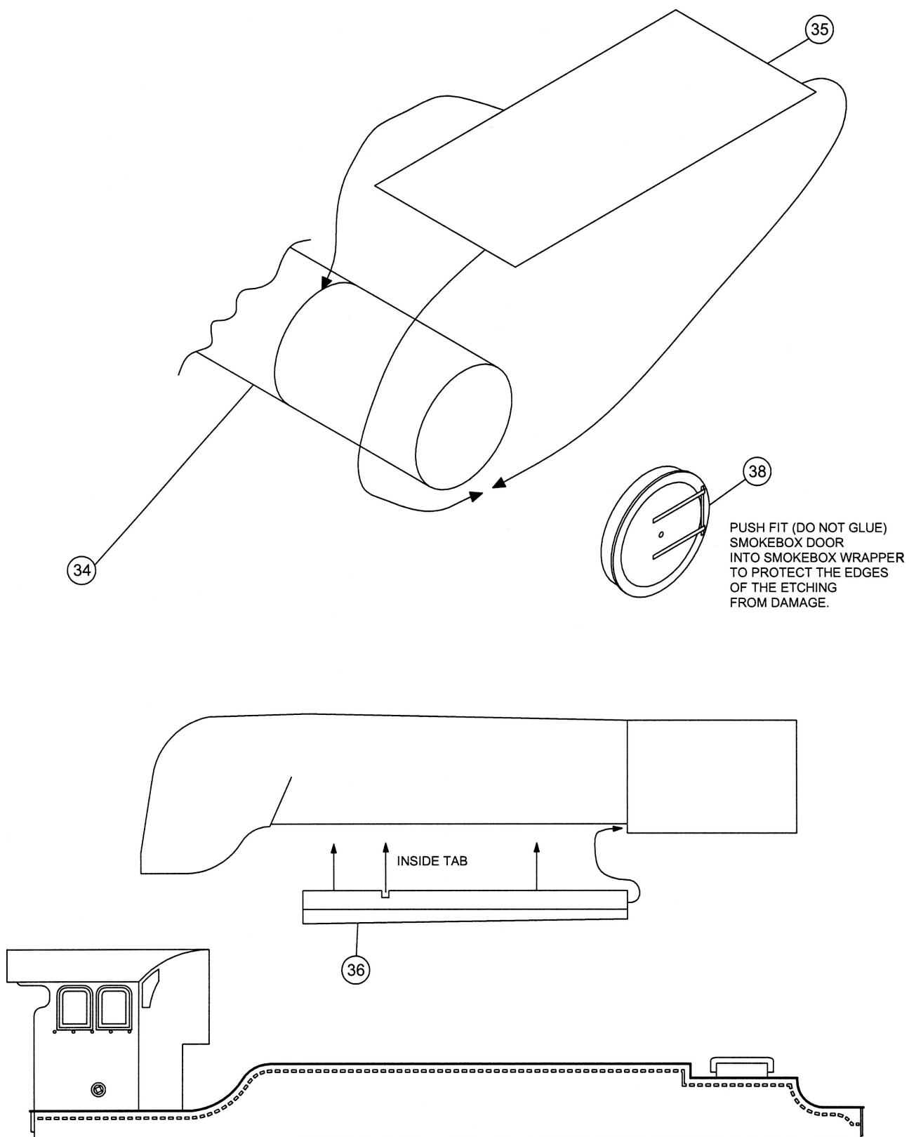
FIG. 3. BOILER PREPARATION.
